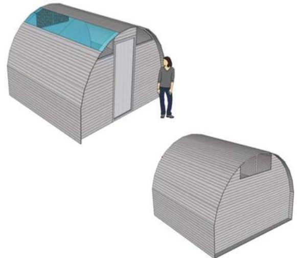
Figure 2: Design of mobile house (floor area: 9 x 12 feet, height at centre 8 feet)
